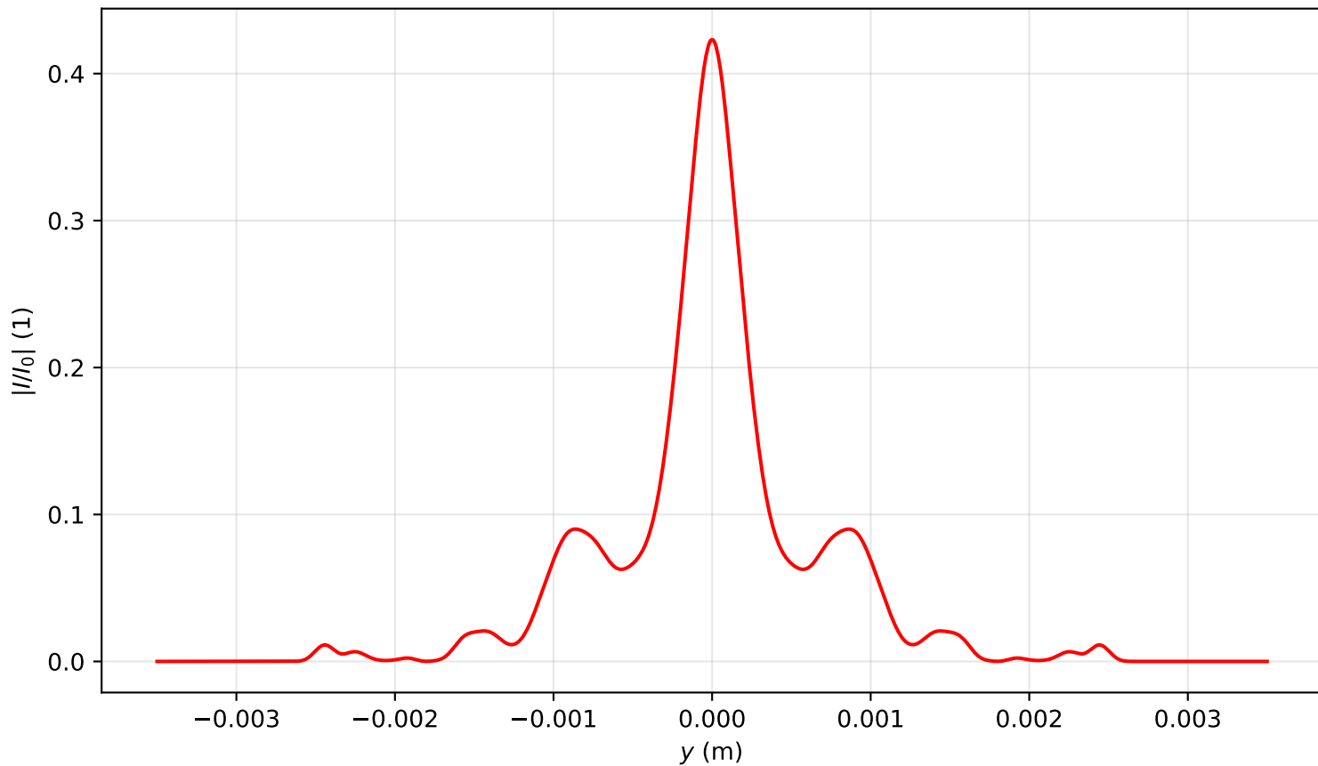
Intensity profile I(x = 0, y, z = 2.388)/I_0 , \text{Pin}=5.5\text{Pcr} , artificial time
